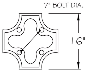
BASE DETAIL
