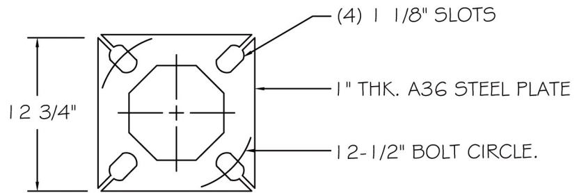
BASE PLATE
